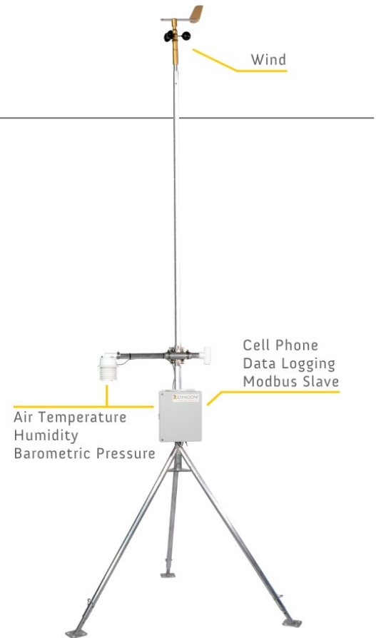
Shown with optional tripod and aspirator.
